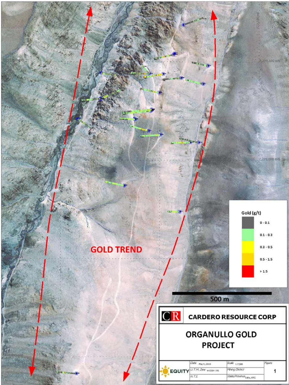
Figure 1: Map of Julio Verne area, showing drill hole traces from historical drilling.
